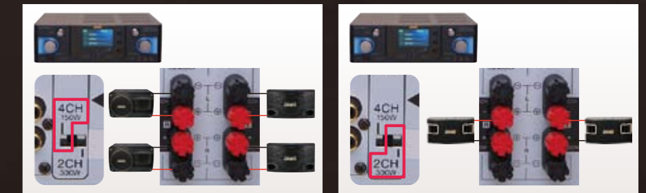
● How to connect (150W × 4CH Mode) ● How to connect (300W × 2CH Mode)
