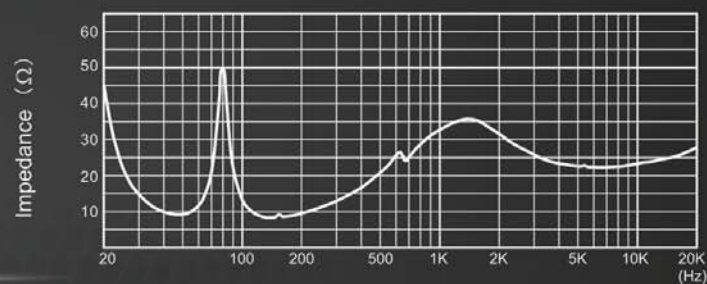
IMPEDANCE FREQUENCY RESPONSE
