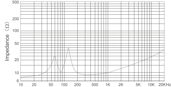
IMPEDANCE FREQUENCY RESPONSE
